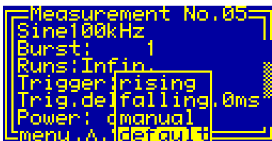
Fig. 18. Setting the trigger slope in the dialog box "Measurement".
