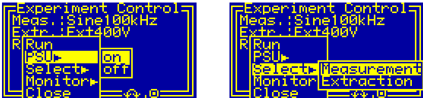
Fig. 42. Start menu of the dialog box "Experiment Control". The figure shows the different submenus of the start menu.
