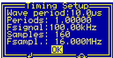
Fig. 14. Dialog box "Timing Setup".
