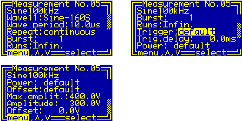
Fig. 9. Dialog box "Measurement".
