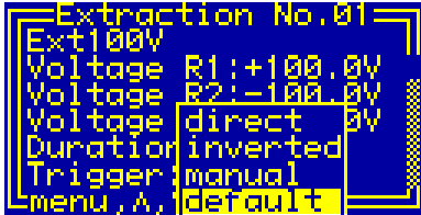
Fig. 27. Setting the trigger slope in the dialog box "Extraction".
