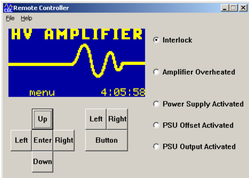
Fig. 56. Utility RemoteControl.
