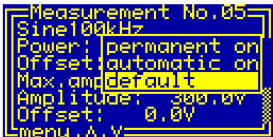
Fig. 20. Setting the activation of the amplifier's power supplies in the dialog box "Measurement".
