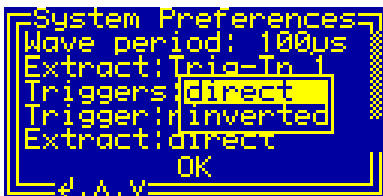
Fig. 31. Setting the pulse polarity controlling the shared trigger input 1 in the dialog box "System Preferences".
