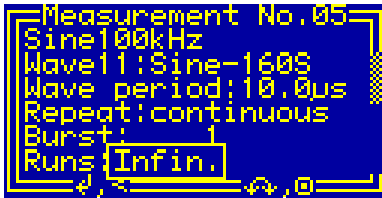
Fig. 17. Setting the number of waveform repetitions in the dialog box "Measurement".
