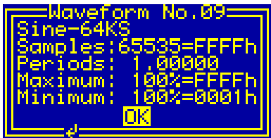
Fig. 6. Dialog box "Waveform Detail".
