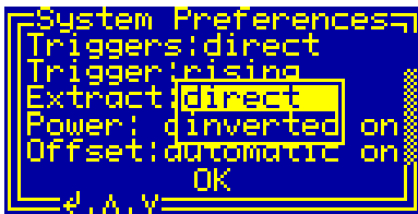
Fig. 33. Setting the polarity of the extraction pulses in the dialog box "System Preferences".
