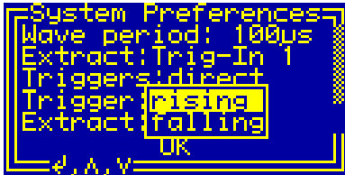
Fig. 32. Setting the trigger slope in the dialog box "System Preferences".
