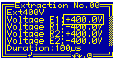
Fig. 26. Setting the extraction voltage in the dialog box "Extraction".
