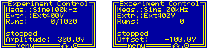
Fig. 41. Dialog box "Experiment Control". Two different views of the dialog box that correspond to different settings.
